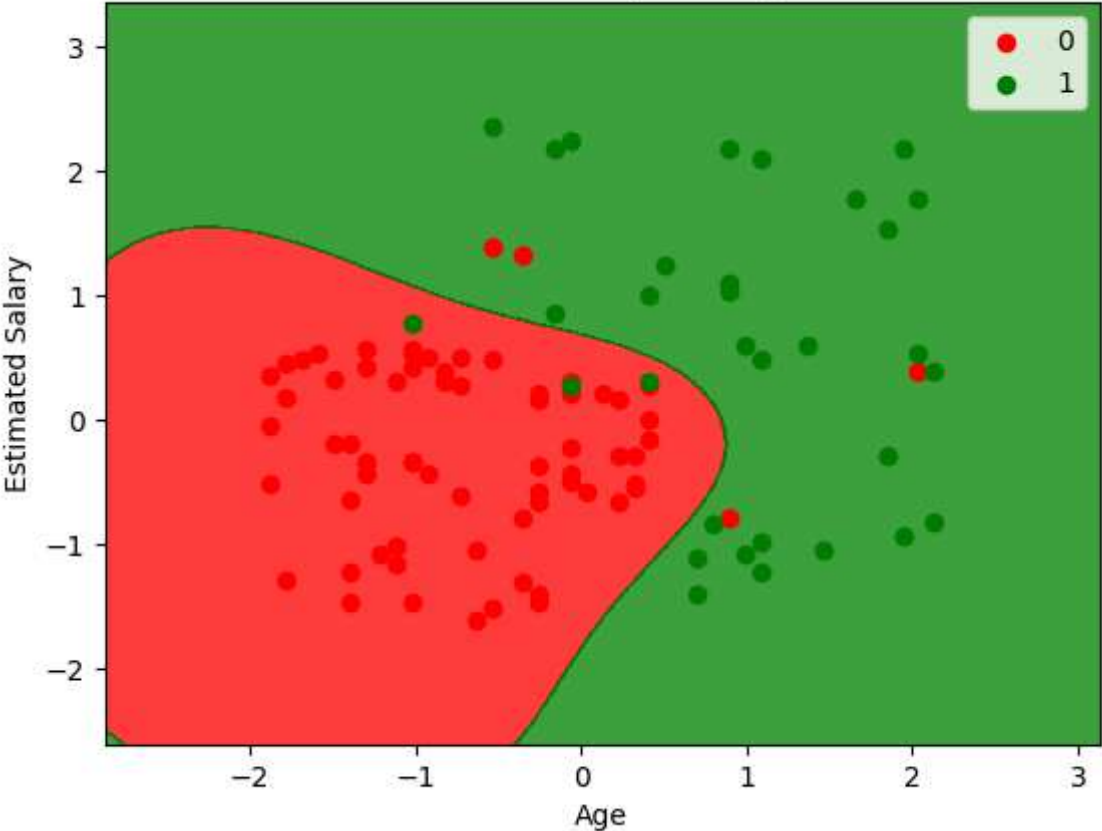
Kernel SVM (Test set)
